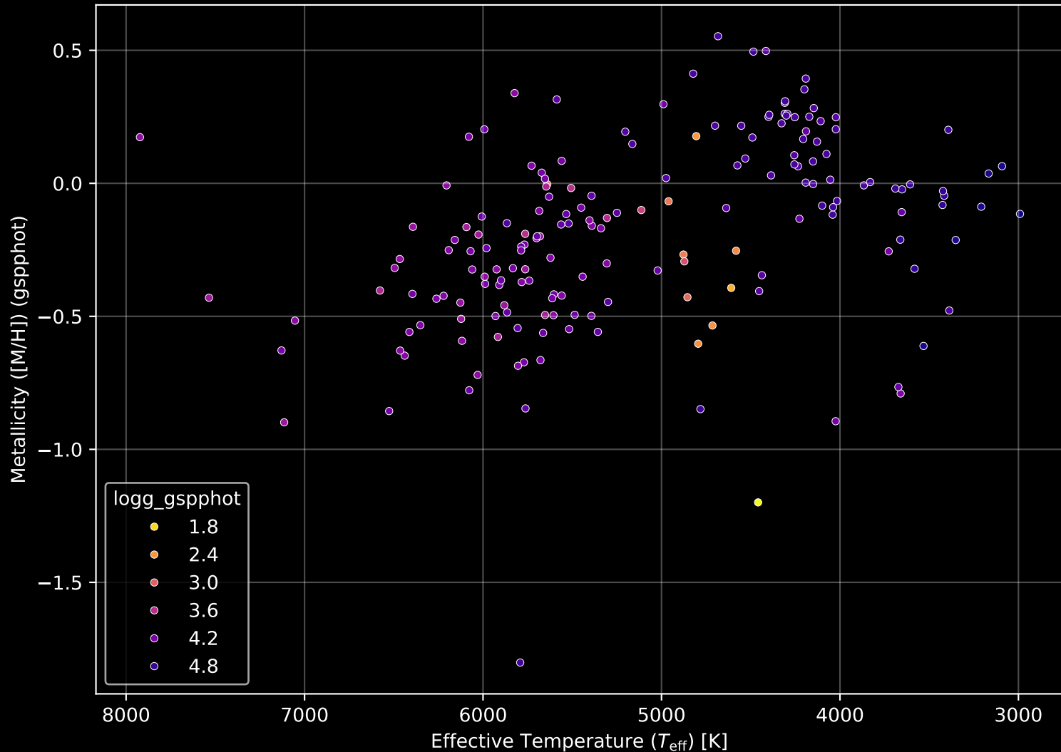
APOGEE DR17 Field: [K2_C3_047-51] Stellar Population Parameters (n= 180)
