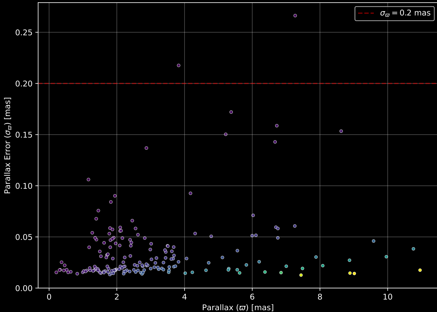
APOGEE DR17 Field: [K2_C3_047-51] Parallax Quality (n= 180)
