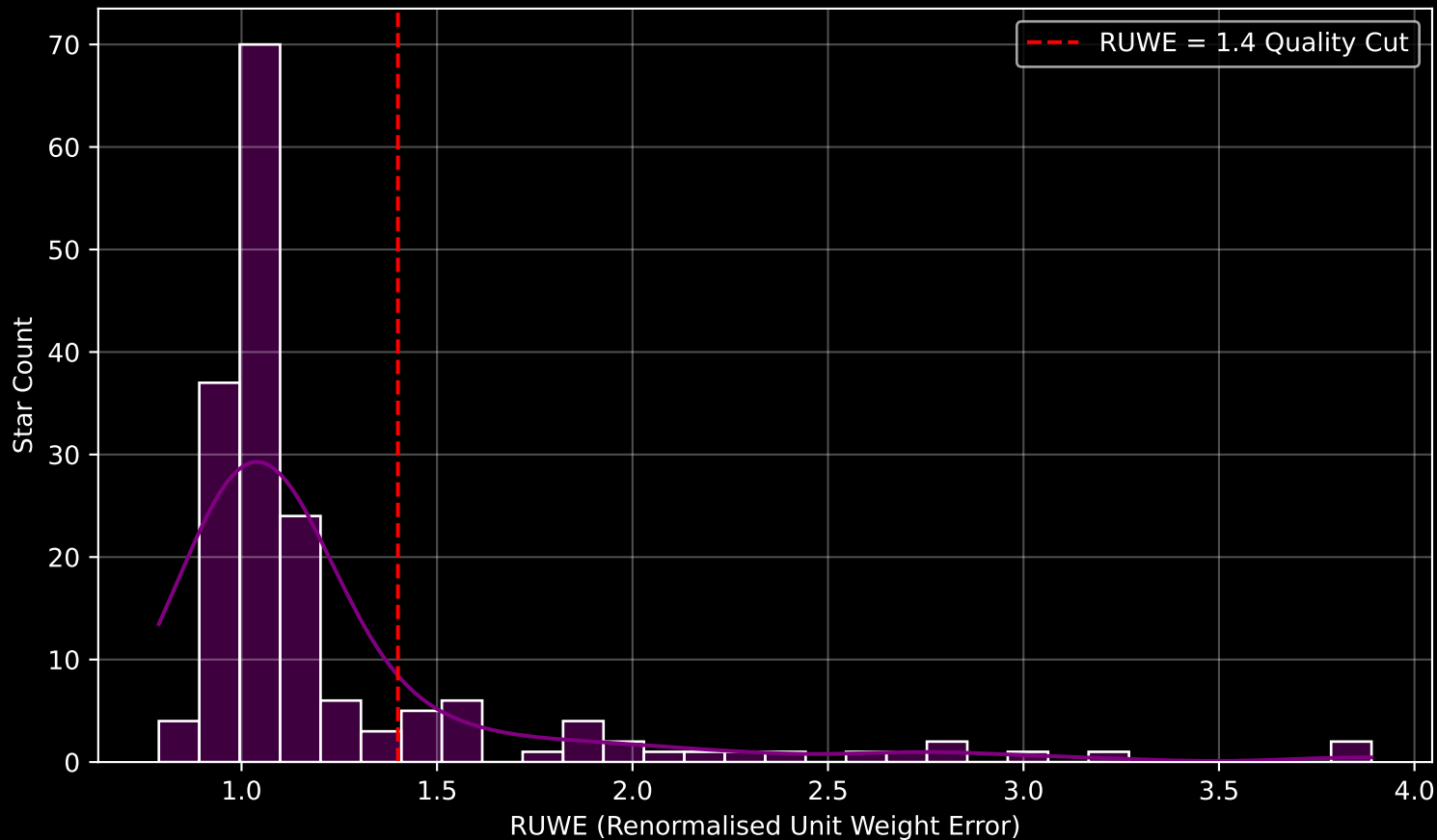
GAPOGEE DR17 Field [K2_C3_047-51] RUWE Distribution (n= 174)
