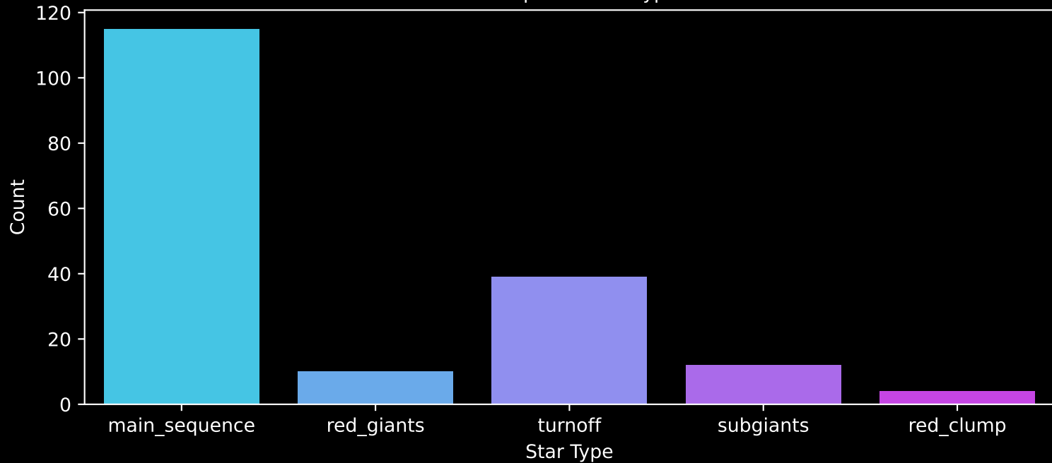
APOGEE DR17 Field: [K2_C3_047-51] Count plot of Star Type
