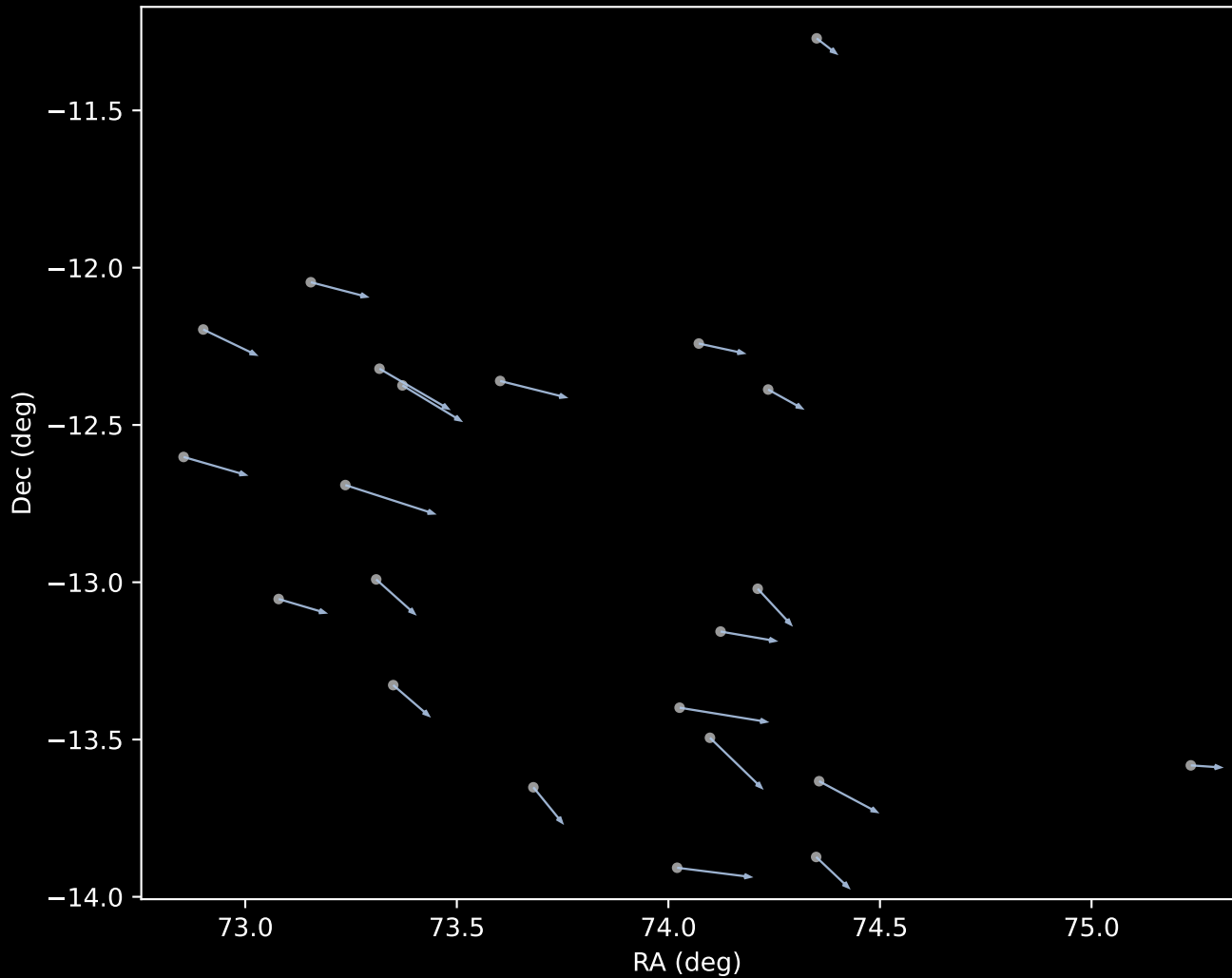
APOGEE DR17 Cluster 1 Proper Motion Vectors (n=22)
