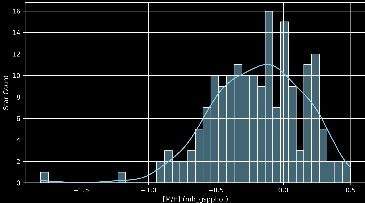
APOGEE DR17 Field: [K2_C3_047-51 [M/H] (mh_gspphot) (n= 179)
