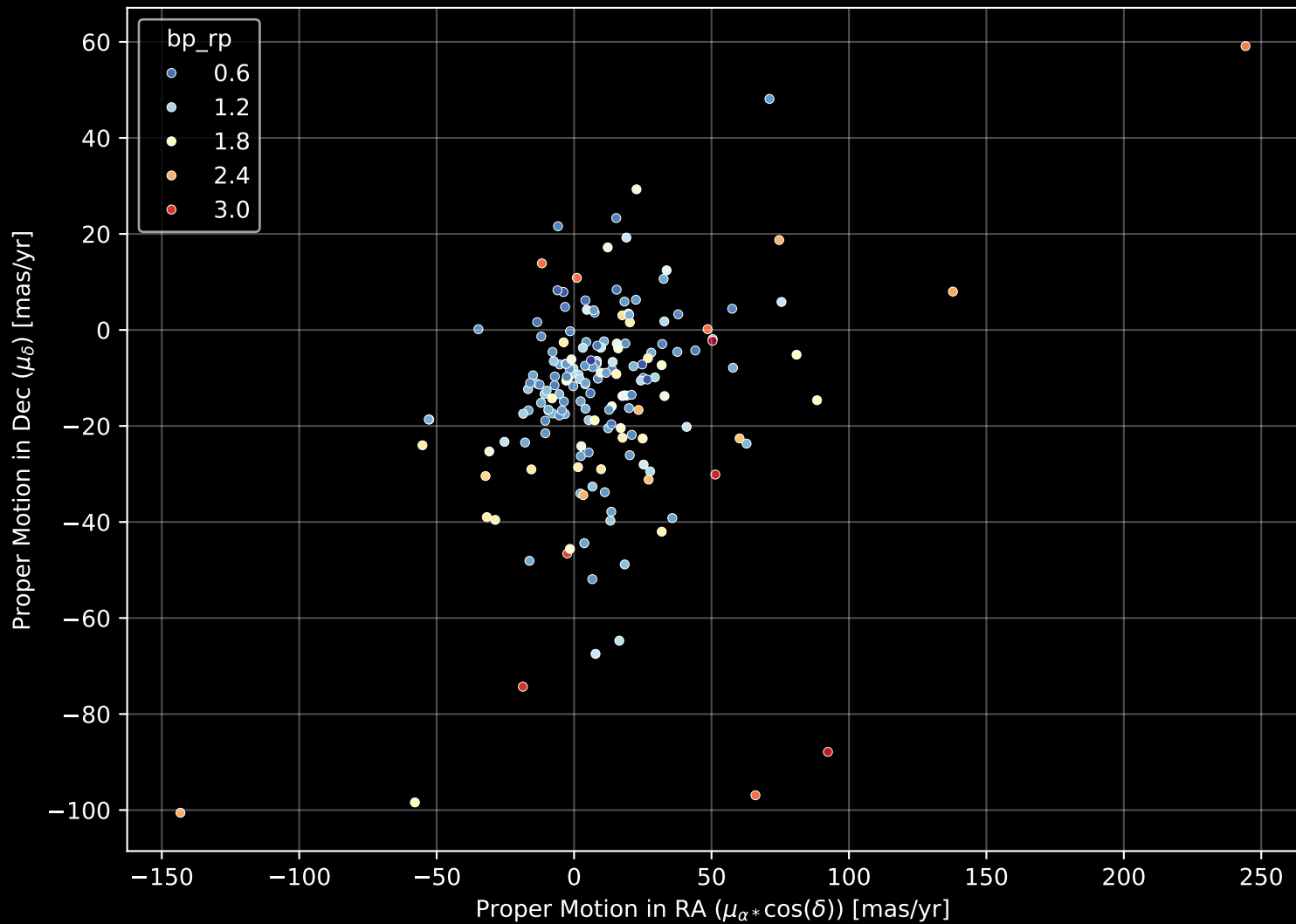
APOGEE DR17 Field: [K2_C3_047-51] Proper Motion Diagram (n= 180)
